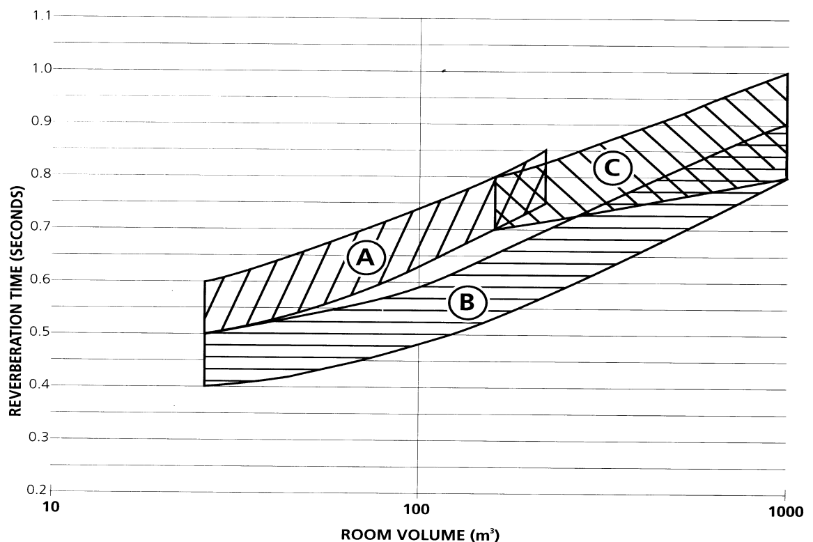
Figure 7: Reverberation times
